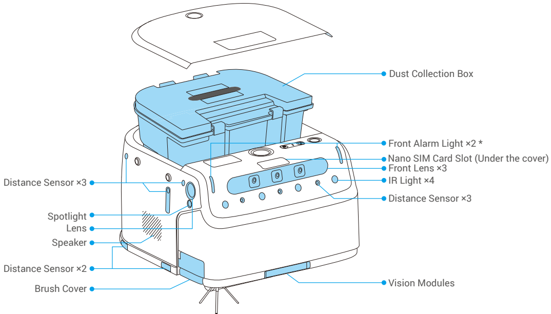
Vacuum Version
